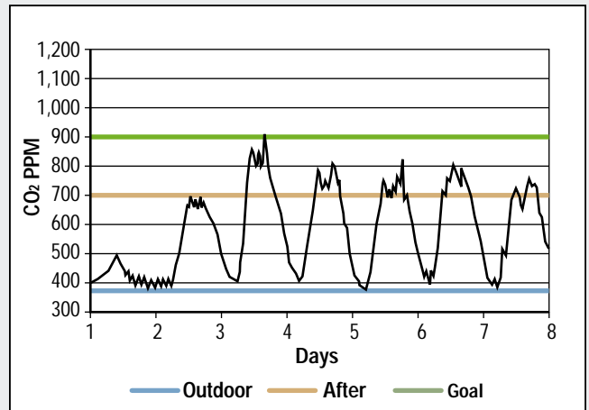
FIGURE 4. CO 2 trends logged after a CO 2 -control system was installed.
