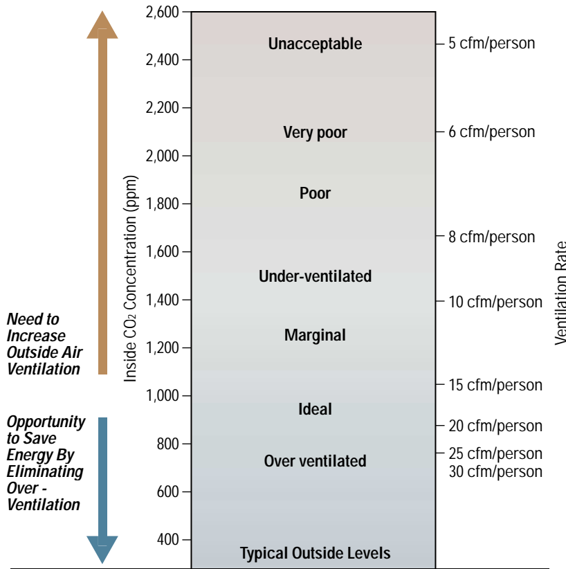
FIGURE 1. The relationship between CO 2 and ventilation rates, assuming adult occupants sitting or involved in office-type activity.
