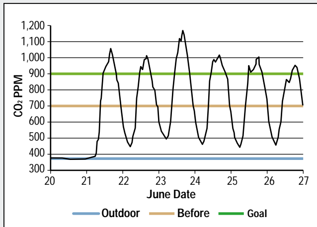
FIGURE 3. Initial CO 2 measurements.
