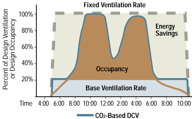
FIGURE 2. A graphic representation of potential energy savings. The dashed line shows a scheduled ventilation strategy for maximum occupancy.
